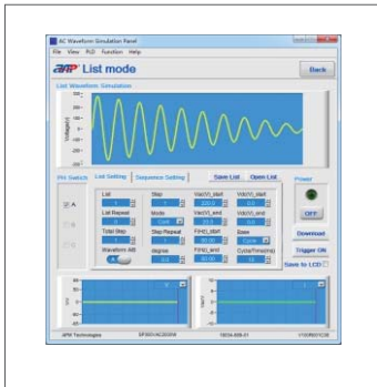
List mode interface
