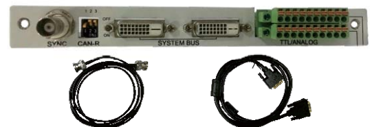
(5) Analog I/O & multiphase link card & cables
