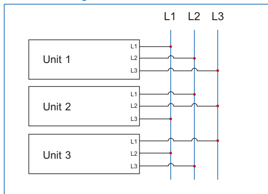
Phase balancing connection for three 12kW units
